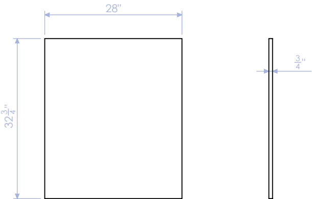
HTW-100-FC-4 FINISH PANEL 3/4" WHITE OAK PLY QTY: 1
