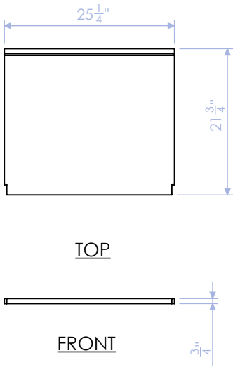
HTW-100-DC-5 CABINET BOTTOM 3/4" WHITE OAK PLY QTY: 2
