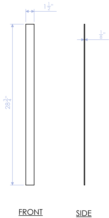
HTW-100-MC-9 VERTICAL FLATBAR 1 1/2" X 1/8" FLATBAR QTY: 1
