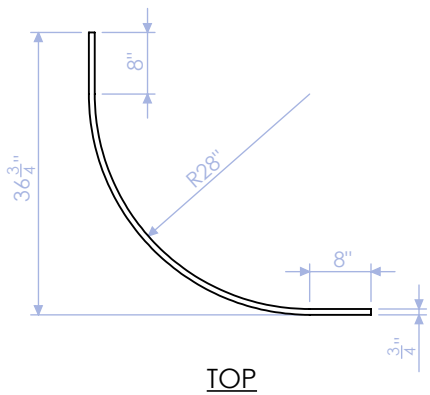
HTW-100-CW-4 INSIDE PANEL 3/4" KERF CORE QTY: 1
