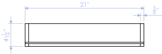
HTW-100-FC-TD-4 DRAWER BOX: SIDE 5/8" PLY QTY: 2
