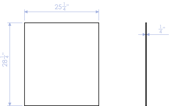
HTW-100-DC-4 CABINET BACK 1/4" WHITE OAK PLY QTY: 2
