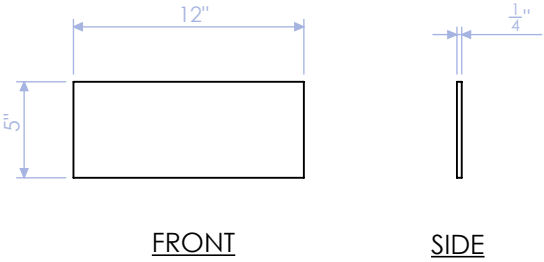
HTW-100-MC-4 FRONT RISER 1/4" STEEL PLATE QTY: 1
