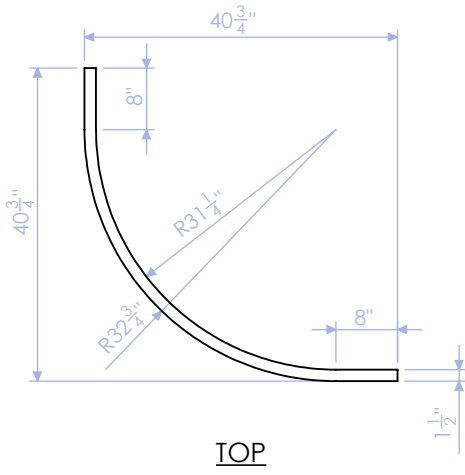
HTW-100-CW-7 TOP CAP 3/4" PLY QTY: 1
