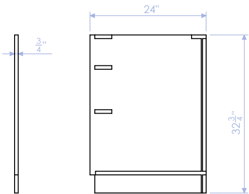
HTW-100-FC-1 CABINET SIDE: LEFT 3/4" WHITE OAK PLY QTY: 1
