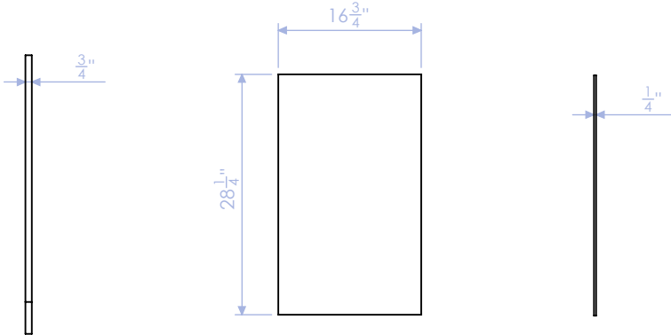
HTW-100-FC-3 CABINET BACK 1/4" WHITE OAK PLY QTY: 1
