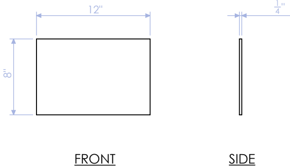
HTW-100-MC-4 ADA RISER 1/4" STEEL PLATE QTY: 1
