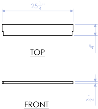
HTW-100-DC-6 FRONT STRETCHER 3/4" WHITE OAK PLY QTY: 2
