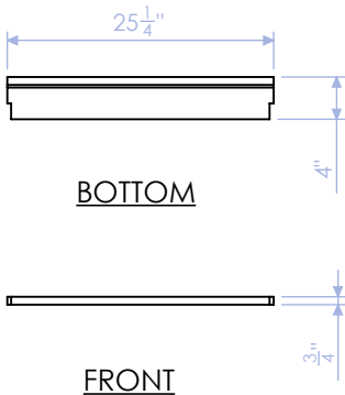
HTW-100-DC-7 BACK STRETCHER 3/4" WHITE OAK PLY QTY: 2
