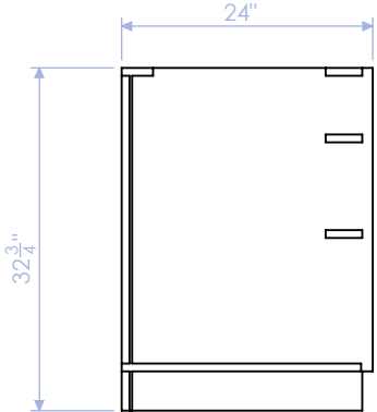
HTW-100-FC-2 CABINET SIDE: RIGHT 3/4" WHITE OAK PLY QTY: 1
