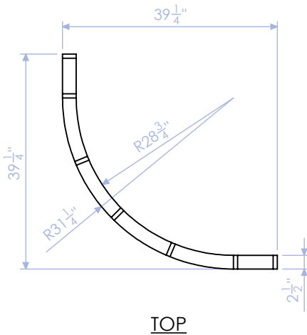
HTW-100-CW-5 TOP/BOTTOM PROFILE 3/4" PLY QTY: 2
