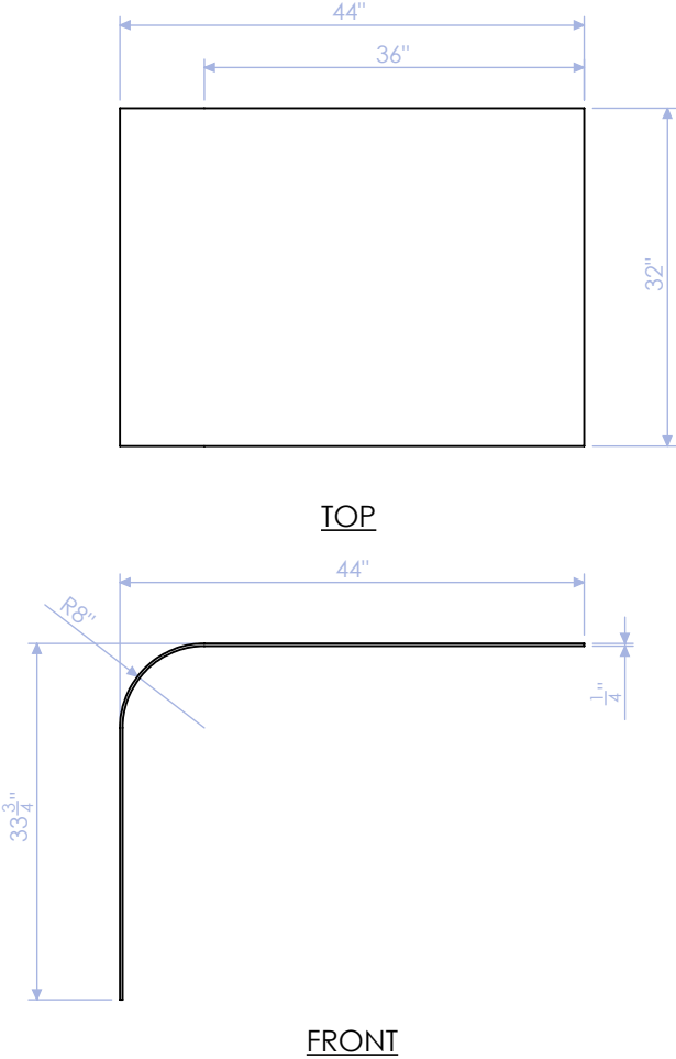
HTW-100-MC-1 ADA COUNTERTOP 1/4" STEEL PLATE QTY: 1
