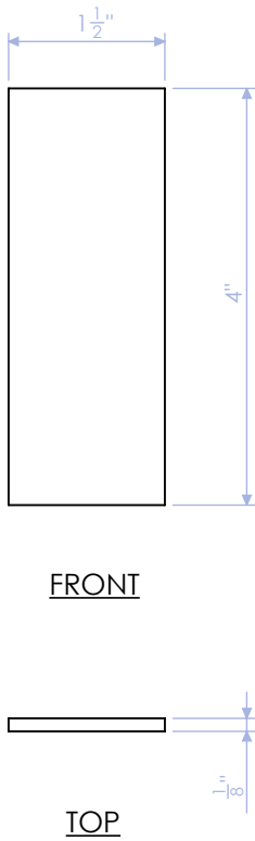
HTW-100-MC-12 ADA RISER TAB 1 1/2" X 1/8" FLATBAR QTY: 1
