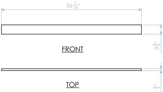
HTW-100-DC-9 TOE KICK 3/4" WHITE OAK PLY QTY: 1
