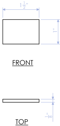
HTW-100-MC-11 FRONT RISER TAB 1 1/2" X 1/8" FLATBAR QTY: 1
