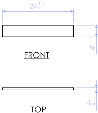
HTW-100-DC-8 NAILER 3/4" WHITE OAK PLY QTY: 4
