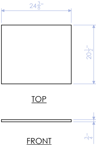
HTW-100-DC-11 SHELF 3/4" WHITE OAK PLY QTY: 4
