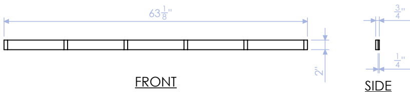
DELB-RF-6 FRONT STRINGER 3/4" PLY QTY:2
