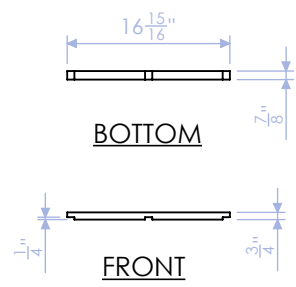
DELB-LB-8 TOP CAP: SHORT SIDE 3/4" PLY QTY:1
