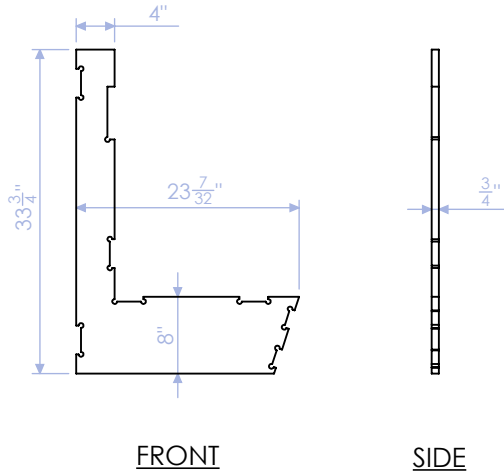
DELB-RF-2 STANDARD RIB 3/4" PLY QTY:6
