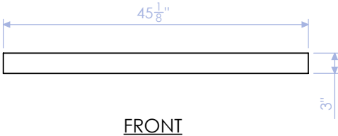
DELB-LF-4 FRENCH CLEAT STRINGER 3/4" PLY QTY:1
