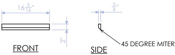
DELB-LB-6 FRENCH CLEAT: SHORT SIDE 3/4" PLY QTY:1
