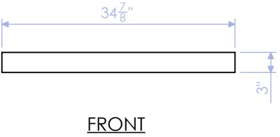
DELB-CTF-3 FRENCH CLEAT STRINGER 3/4" PLY QTY:1
