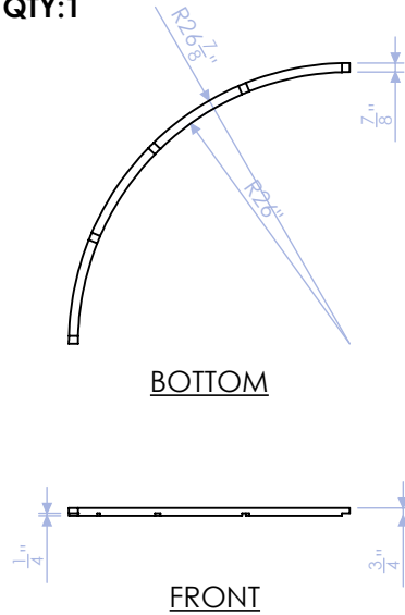
DELB-RB-10 CURVED TOP CAP 3/4" PLY QTY:1
