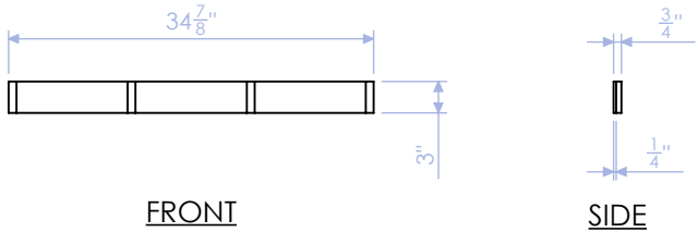
DELB-CTF-2 STANDARD STRINGER 3/4" PLY QTY:5
