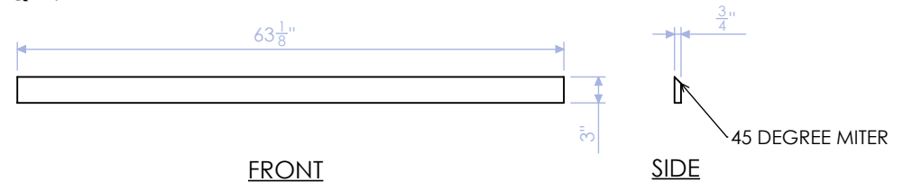
DELB-RF-4 FRENCH CLEAT STRINGER 3/4" PLY QTY:1
