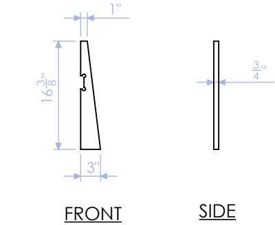
DELB-RB-1 STANDARD RIB 3/4" PLY QTY:10
