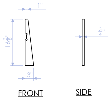
DELB-LB-1 STANDARD RIB 3/4" PLY QTY:8
