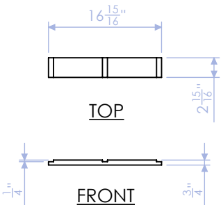
DELB-RB-12 BOTTOM CAP: SHORT SIDE 3/4" PLY QTY:1
