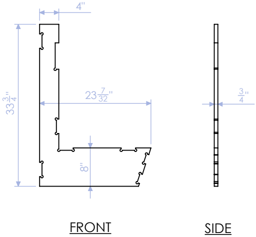
DELB-CTF-1 STANDARD RIB 3/4" PLY QTY:4
