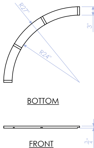
DELB-COF-4 BACK STRINGER 3/4" PLY QTY:2
