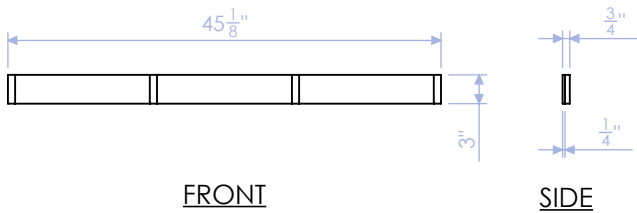
DELB-LF-3 STANDARD STRINGER 3/4" PLY QTY:5
