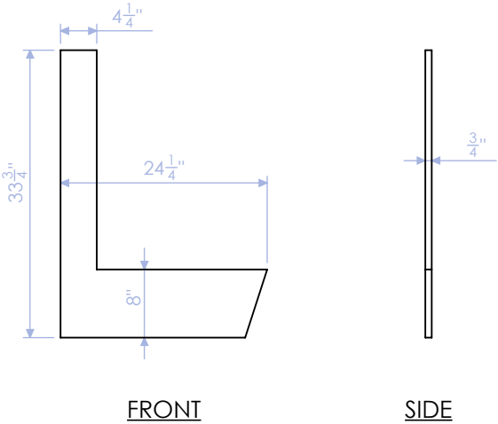
DELB-LF-1 FINISH PANEL 3/4" MDF: PAINTED QTY:1
