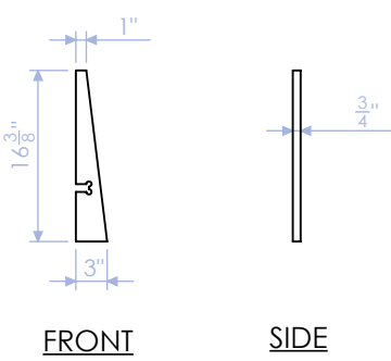
DELB-LB-2 CORNER RIB 3/4" PLY QTY:5
