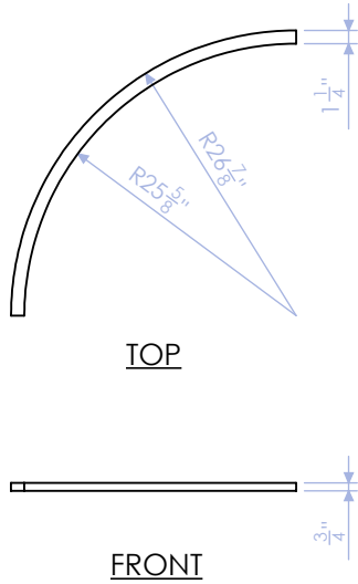
DELB-RB-9 CURVED STRINGER 3/4" PLY QTY:1
