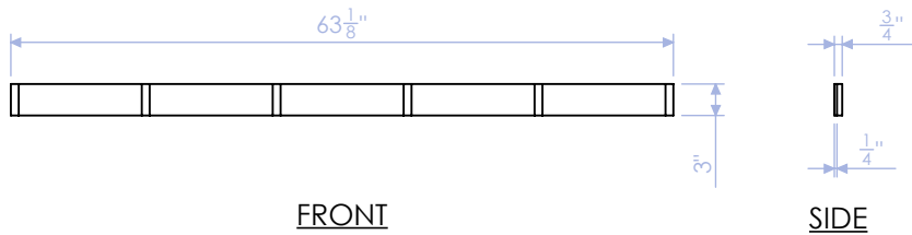
DELB-RF-3 STANDARD STRINGER 3/4" PLY QTY:5
