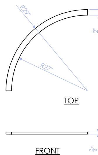
DELB-COF-5 MIDDLE STRINGER 3/4" PLY QTY:2
