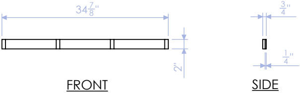
DELB-CTF-5 FRONT STRINGER 3/4" PLY QTY:2
