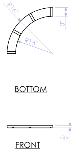
DELB-COF-3 FRONT STRINGER 3/4" PLY QTY:2
