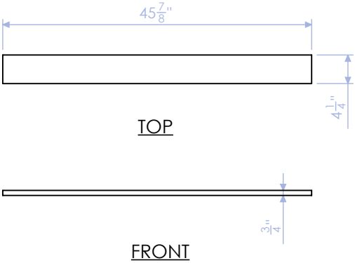
DELB-LF-5 TOP CAP 3/4" MDF: PAINTED QTY: 1
