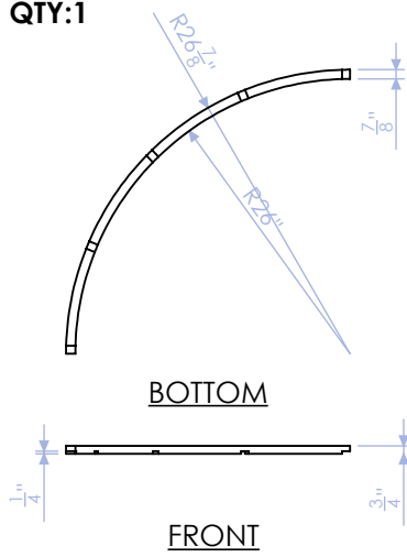
DELB-LB-10 CURVED TOP CAP 3/4" PLY QTY:1
