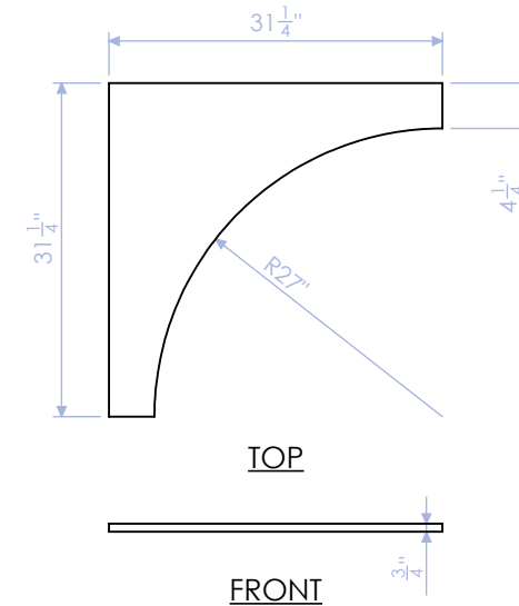
DELB-COF-6 TOP CAP 3/4" MDF: PAINTED QTY:1
