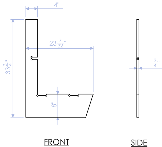
DELB-COF-1 CORNER RIB: OUTSIDE 3/4" PLY QTY:4
