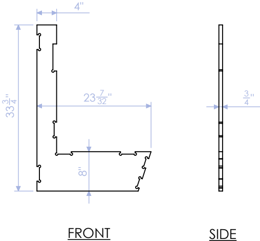
DELB-LF-2 STANDARD RIB 3/4" PLY QTY:4
