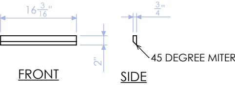
DELB-RB-6 FRENCH CLEAT: SHORT SIDE 3/4" PLY QTY:1
