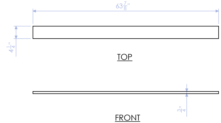
DELB-RF-5 TOP CAP 3/4" MDF: PAINTED QTY:1
