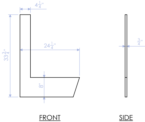
DELB-RF-1 FINISH PANEL 3/4" MDF: PAINTED QTY:1
