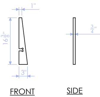
DELB-RB-2 CORNER RIB 3/4" PLY QTY:5
