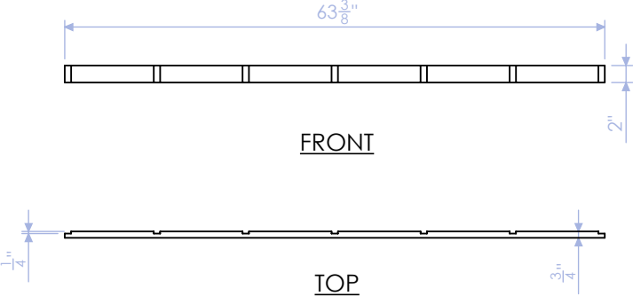
DELB-RB-3 BACK STRINGER: LONG SIDE 3/4" PLY QTY:1
