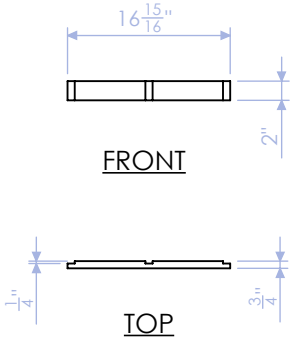
DELB-RB-4 BACK STRINGER: SHORT SIDE 3/4" PLY QTY:1
