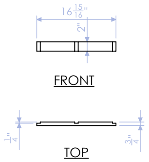
DELB-LB-4 BACK STRINGER: SHORT SIDE 3/4" PLY QTY:1
