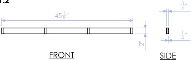
DELB-LF-6 FRONT STRINGER 3/4" PLY QTY:2
