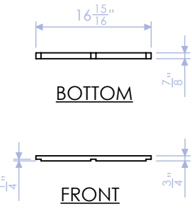
DELB-RB-8 TOP CAP: SHORT SIDE 3/4" PLY QTY:1
