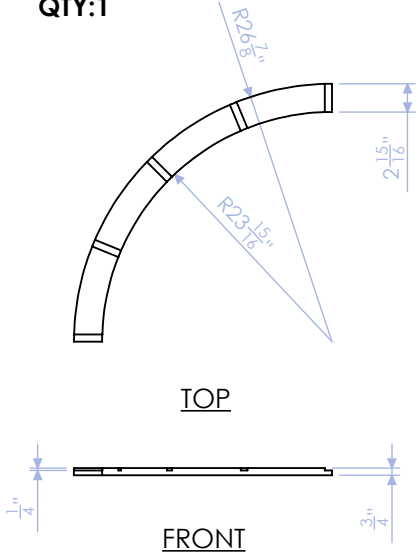
DELB-RB-13 CURVED BOTTOM CAP 3/4" PLY QTY:1
