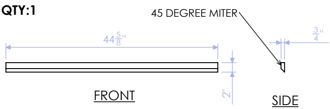
DELB-LB-8 TOP CAP: SHORT SIDE 3/4" PLY QTY:1
