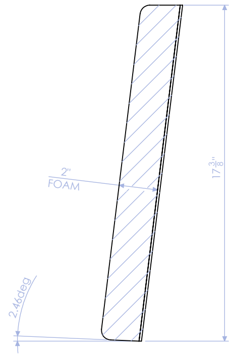
SEAT BACK CROSS SECTION: TYP
