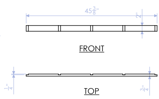
DELB-LB-3 BACK STRINGER: LONG SIDE 3/4" PLY QTY:1
