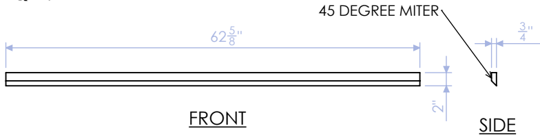
DELB-RB-5 FRENCH CLEAT: LONG SIDE 3/4" PLY QTY:1
