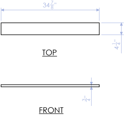
DELB-CTF-4 TOP CAP 3/4" MDF: PAINTED QTY:1
