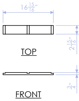
DELB-LB-12 BOTTOM CAP: SHORT SIDE 3/4" PLY QTY:1
