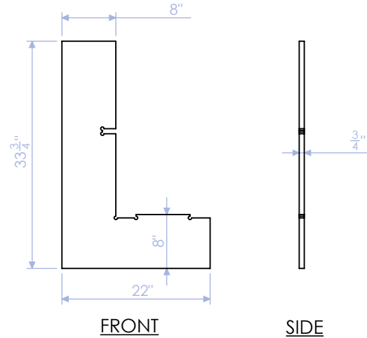
DELB-COF-2 CORNER RIB: MIDDLE 3/4" PLY QTY:4
