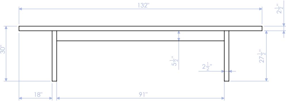
FRONT
