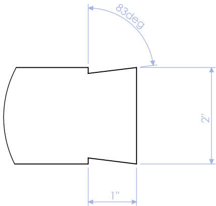
DETAIL AA SLIDING DOVETAIL JOINT SCALE_1 : 2
