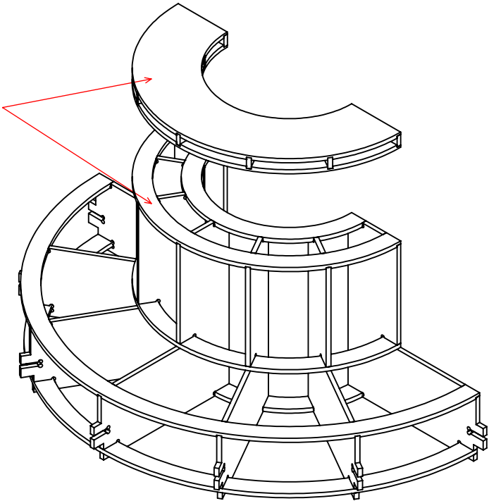
ISOMETRIC
