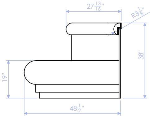
SIDE
