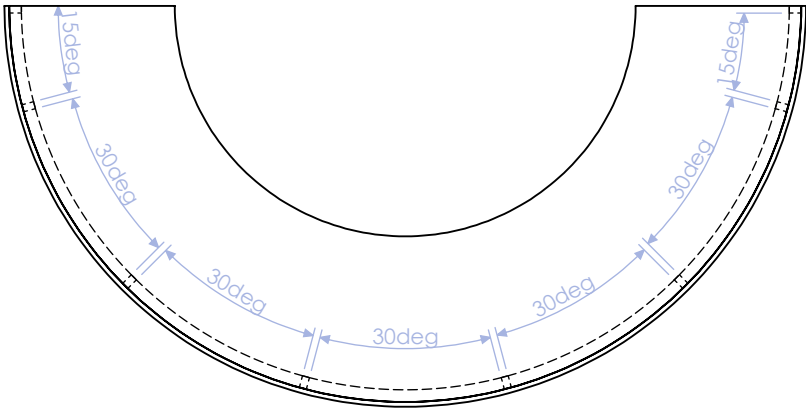
TOP: RIB LAYOUT
