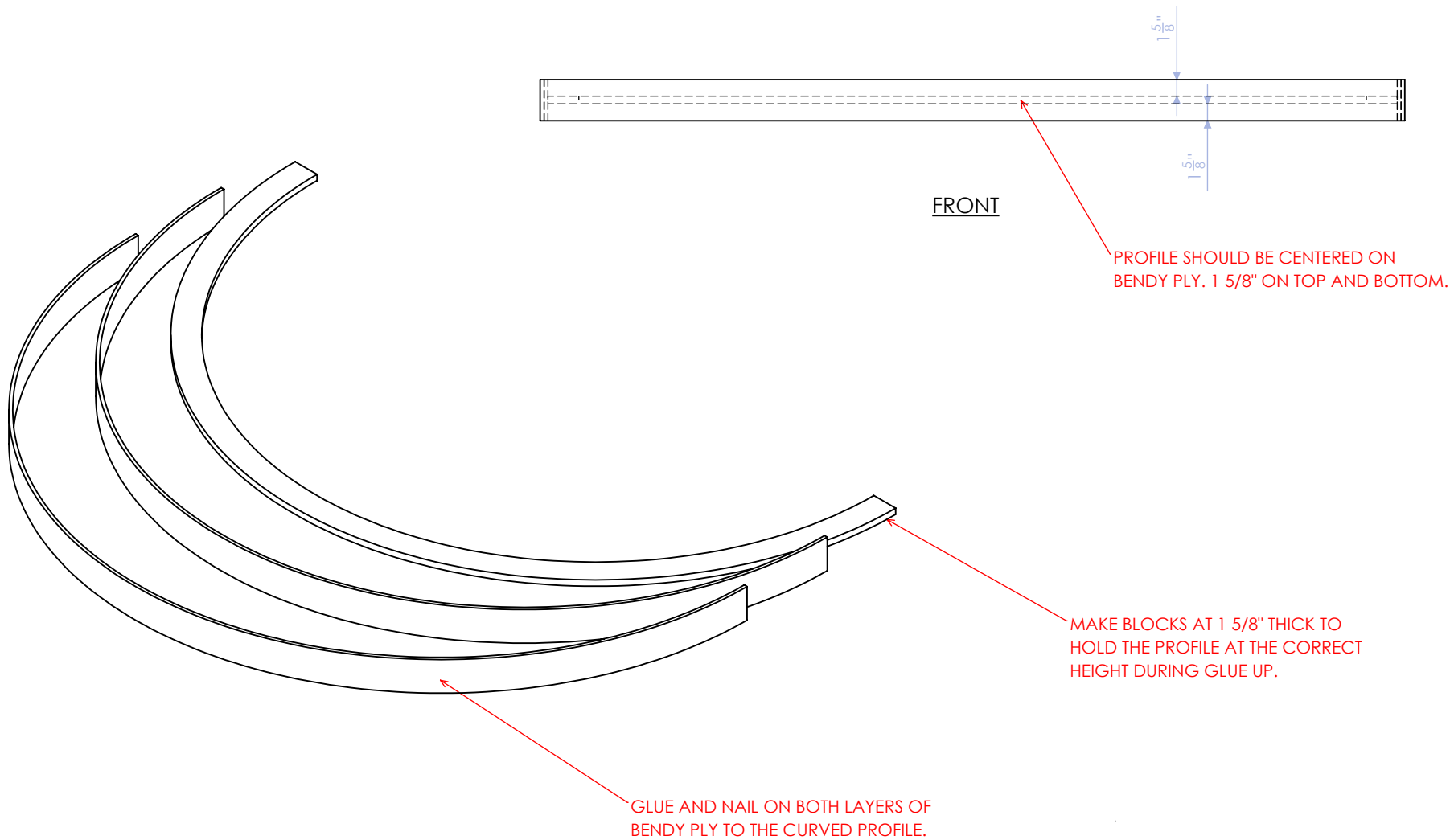
ISOMETRIC: EXPLODED
