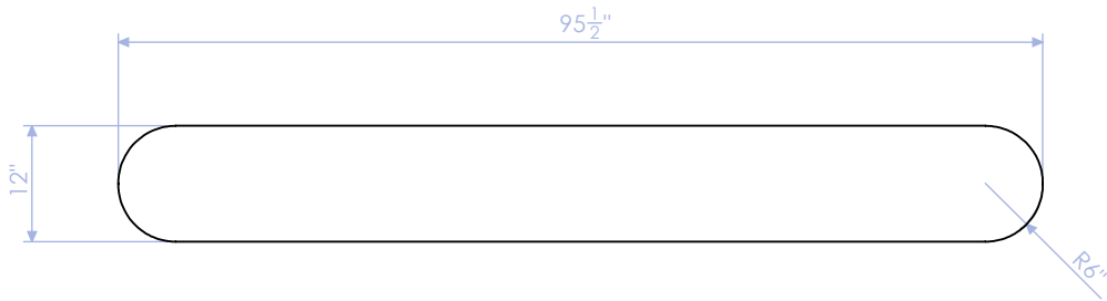
FRONT
