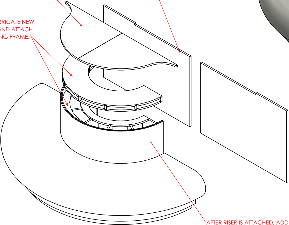
EXPLODED
