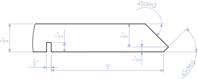
DETAIL AB *STANDARD END DETAIL FOR LA-100-FRAME-1 AND 2 SCALE_1 : 1.5
