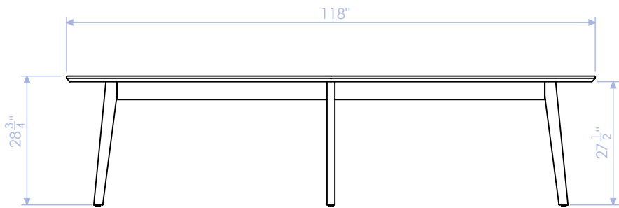
FRONT
