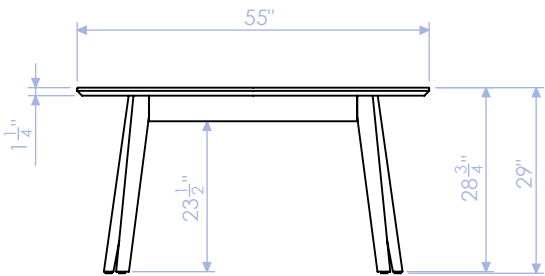
SIDE
