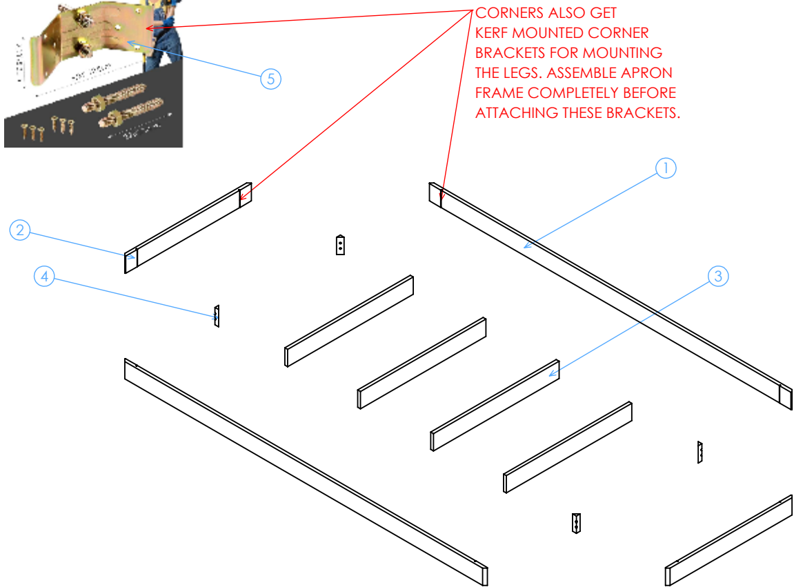
EXPLODED
