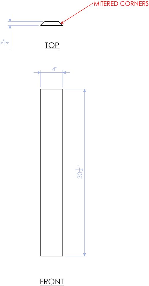
GPH-100-LEP-2 NARROW PANEL 3/4" ASH VENEER PLY QTY: 2
