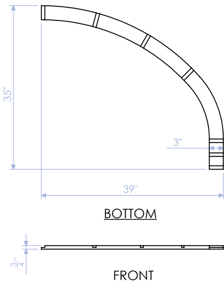
GPH-100-LF-11 LOWER PROFILE: FRONT 3/4" PLY QTY: 1
