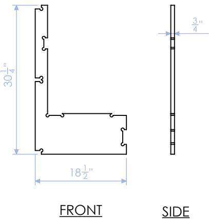
GPH-100-LF-6 BACK PROFILE 3/4" PLY QTY: 3
