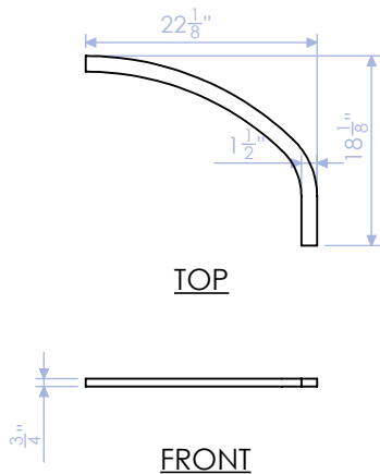
GPH-100-RSF-4 BOTTOM STRINGER 3/4" PLY QTY: 1
