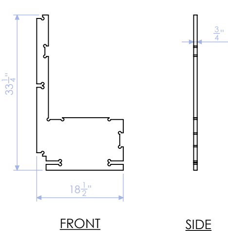
GPH-100-LF-12 BACK TOE KICK 2 LAYERS OF 3/8" BENDY PLY QTY: 1
