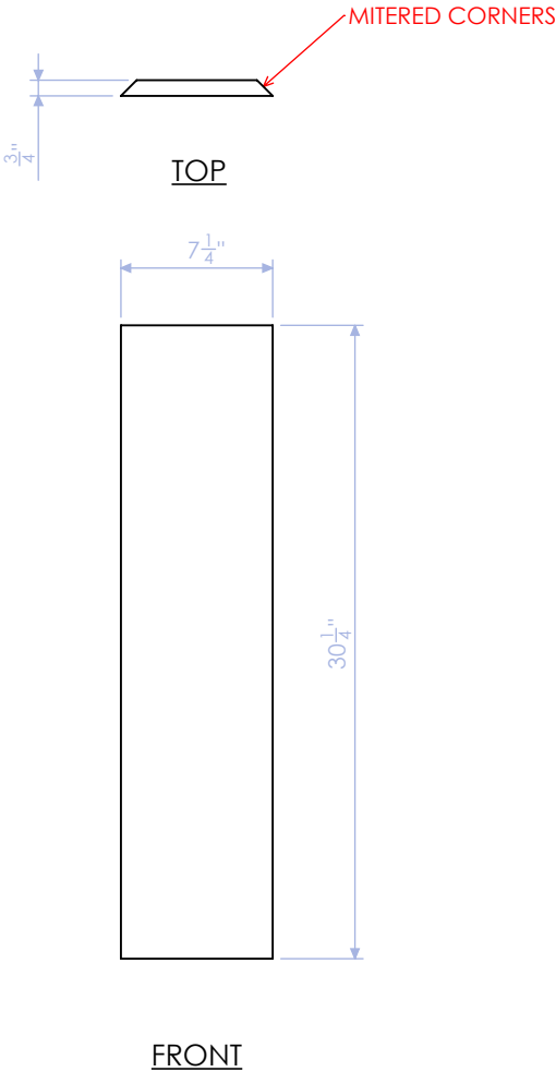
GPH-100-LEP-1 WIDE PANEL 3/4" ASH VENEER PLY QTY: 2
