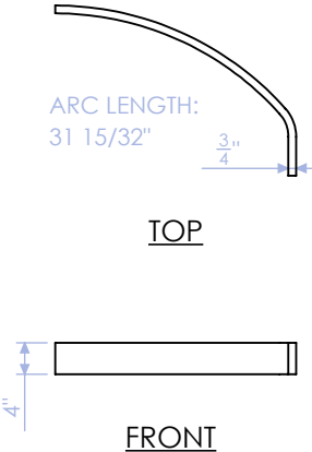
GPH-100-RF-13 FRONT TOE KICK 2 LAYERS OF 3/8" BENDY PLY QTY: 1
