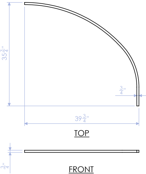
GPH-100-RF-10 LOWER PROFILE: BACK 3/4" PLY QTY: 1
