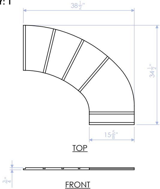
GPH-100-RSF-2 BOTTOM PROFILE 3/4" PLY QTY: 1
