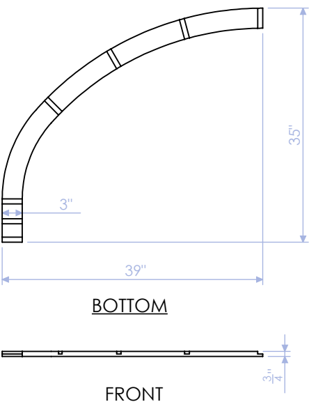
GPH-100-RF-11 LOWER PROFILE: FRONT 3/4" PLY QTY: 1
