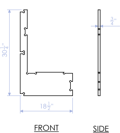
GPH-100-RF-6 BACK PROFILE 3/4" PLY QTY: 3
