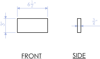
GPH-100-RF-14 SHORT STRINGER 3/4" PLY QTY: 1
