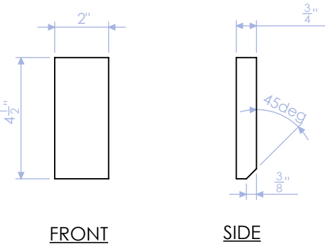
GPH-100-RSB-5 CLEAT HOOK 3/4" PLY QTY: 5
