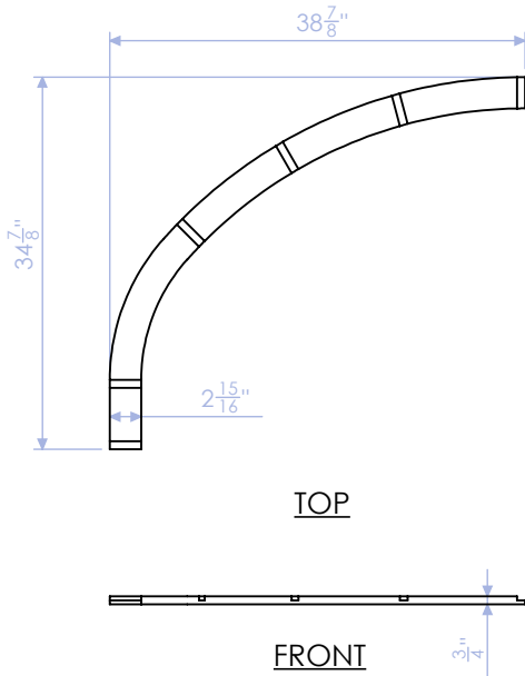
GPH-100-LSB-2 BOTTOM PROFILE 3/4" PLY QTY: 1
