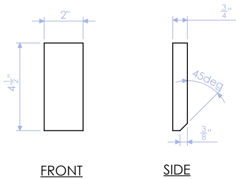
GPH-100-LSB-5 CLEAT HOOK 3/4" PLY QTY: 5
