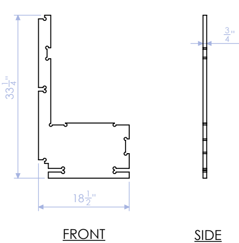
GPH-100-RF-12 BACK TOE KICK 2 LAYERS OF 3/8" BENDY PLY QTY: 1
