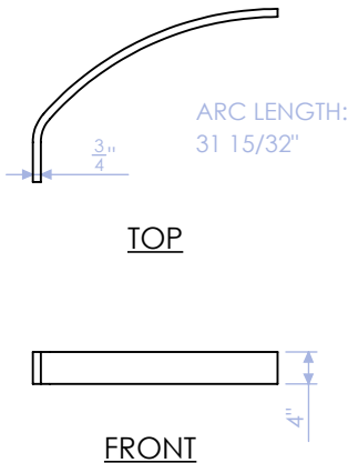
GPH-100-LF-13 FRONT TOE KICK 2 LAYERS OF 3/8" BENDY PLY QTY: 1
