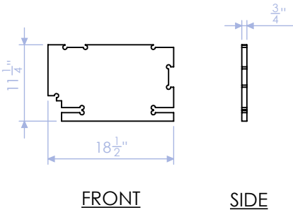
GPH-100-LF-3 SHORT RIB 3/4" PLY QTY: 1
