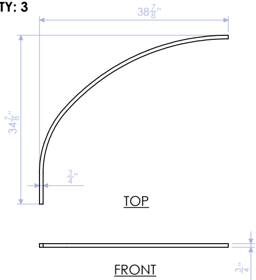
GPH-100-LSB-4 CLEAT PROFILE 3/4" PLY QTY: 3
