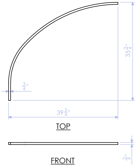
GPH-100-LF-10 LOWER PROFILE: BACK 3/4" PLY QTY: 1
