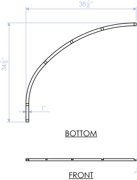
GPH-100-RSB-1 TOP PROFILE 3/4" PLY QTY: 1
