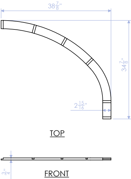
GPH-100-RSB-2 BOTTOM PROFILE 3/4" PLY QTY: 1
