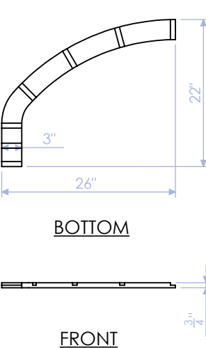
GPH-100-RF-9 TOP PROFILE: FRONT 3/4" PLY QTY: 1
