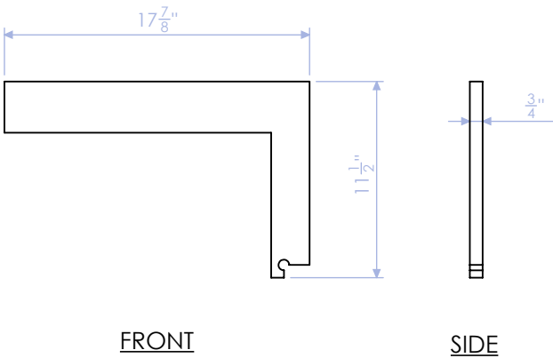
GPH-100-RSF-3 RIB 3/4" PLY QTY: 6
