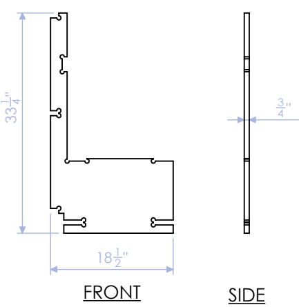
GPH-100-RF-5 BACK WRAP 3/4" KERF CORE QTY: 1
