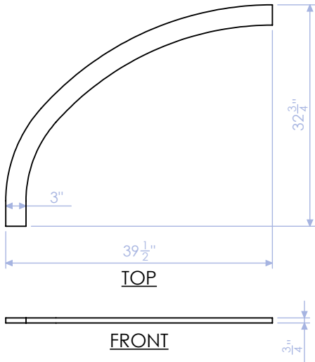
GPH-100-LF-10 LOWER PROFILE: BACK 3/4" PLY QTY: 1
