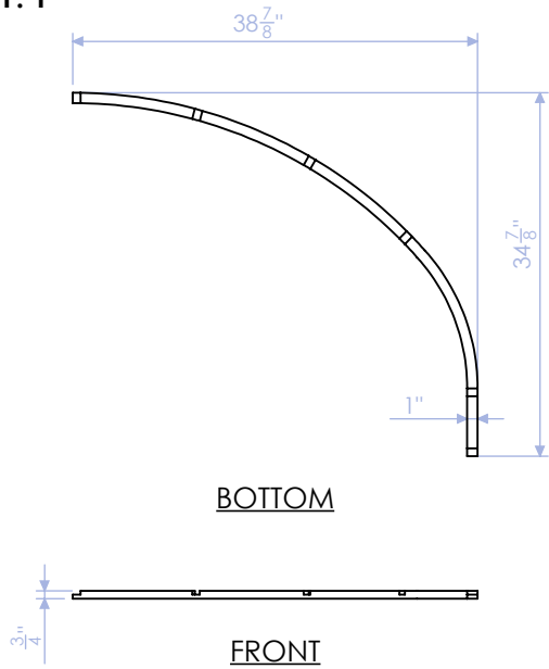
GPH-100-LSB-1 TOP PROFILE 3/4" PLY QTY: 1
