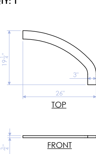
GPH-100-RF-11 LOWER PROFILE: FRONT 3/4" PLY QTY: 1
