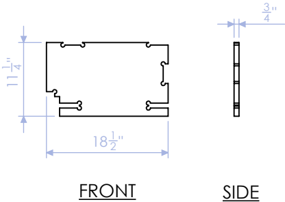
GPH-100-RF-3 SHORT RIB 3/4" PLY QTY: 1
